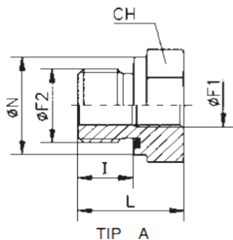
TN141-A Adaptor drept FE-FI
