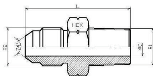
Fiting UNF-NPT - FUNPT
