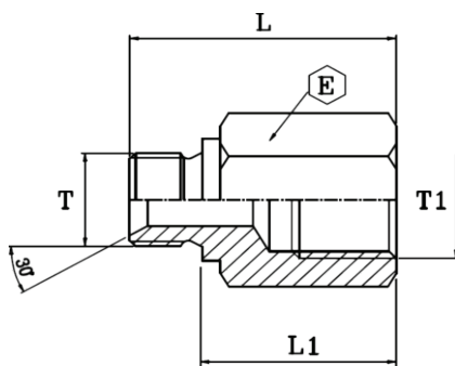
Adaptor BSP FE-FI - BSP-FEFI filet exterior / filet interior con 60 de grade
